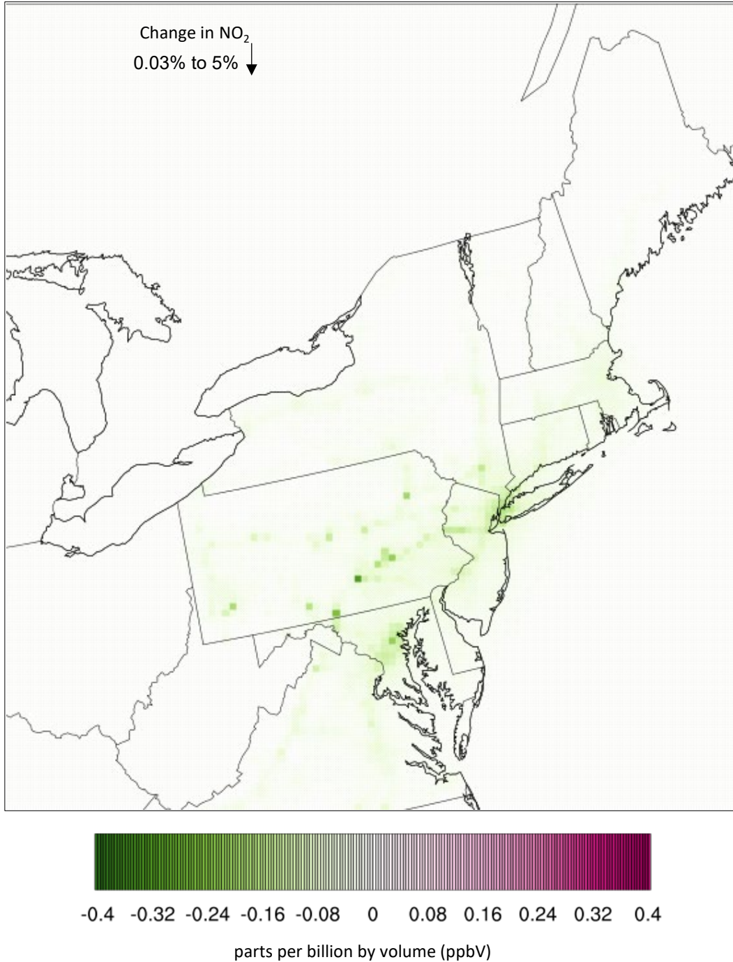
Figure 2c: Estimated Changes in NO 2 Concentrations for Scenario B with a 25% CO 2 Reduction Cap Compared to a No-TCI Reference Scenario in 2032
